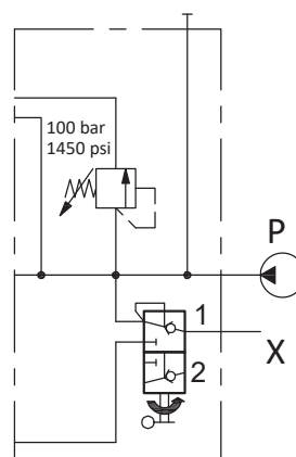
Right inlet
